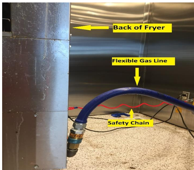
Flexible Gas Connection with Safety Chain
